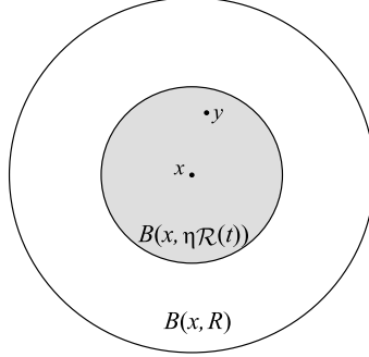
FIG. 6. Illustration to Theorem 5.14.
