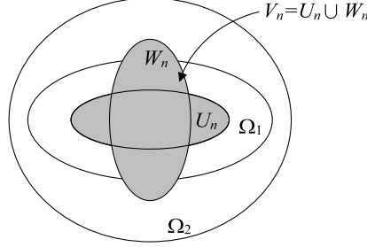
FIG. 1. Sets U_n, W_n, V_n .
