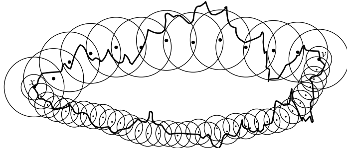
FIG. 8. Two shortest chains of \varepsilon -balls for two distinct values of \varepsilon provide different routes for the diffusion from x to y for two distinct values of time t .
