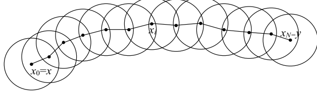
FIG. 7. An \varepsilon -chain connecting x and y .
