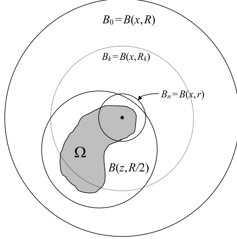
FIG. 2. Balls B_k .
