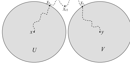
FIG. 5. Illustration to (4.14).
