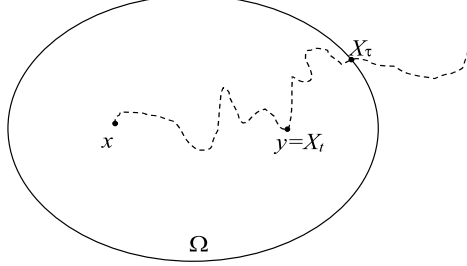
FIG. 3. Illustration to the proof of Lemma 3.12.
