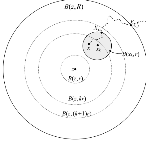
FIG. 4. Exit times from B(x_k, r) and B(z, R) .
