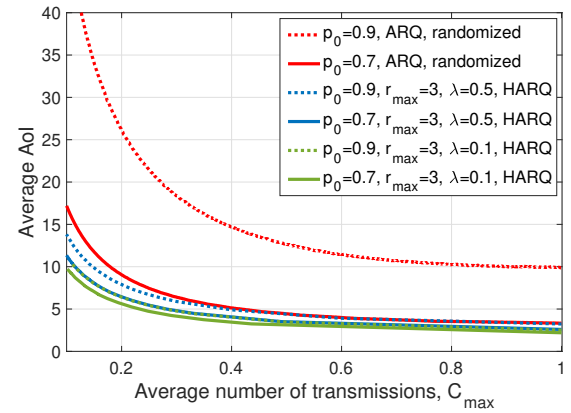
Figure 6. Expected average AoI with respect to C_{max} for ARQ and HARQ protocols for different p_0 and r_{max} values. Time horizon is set to T = 10000 , and the results are averaged over 1000 runs.
