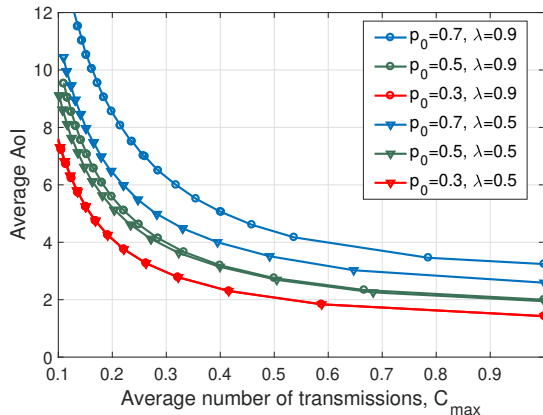
Figure 7. Expected average AoI with respect to C_{max} for HARQ protocols with different g(r) = p_0 \lambda^r values corresponding to different p_0 and \lambda values with r_{max} = 3 . The time horizon is set to T = 10000 , and the results are averaged over 1000 runs.
