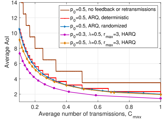
Figure 5. Expected average AoI as a function of C_{max} for ARQ and HARQ protocols for different p_0 values. Time horizon is set to T = 10000 , and the results are averaged over 1000 runs.
