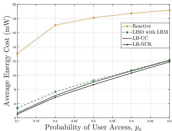
Fig. 7: Average energy cost vs. probability of user access for B = 30 , when K_{max} = 15, M_{max} = 8 .
