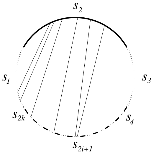
Figure 2: The k -configuration (k \frac{n}{3k-2}, (2k-1) \frac{n}{3k-2}, k \frac{n}{3k-2}, \frac{n}{3k-2}, \dots, \frac{n}{3k-2}) .
