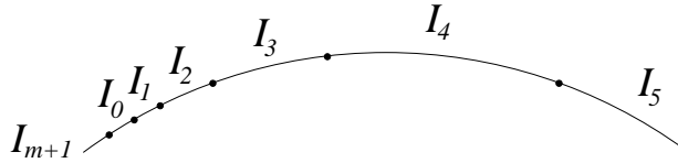
Figure 3: I_0, I_1, \dots, I_{m+1} form a partition of the vertices.
