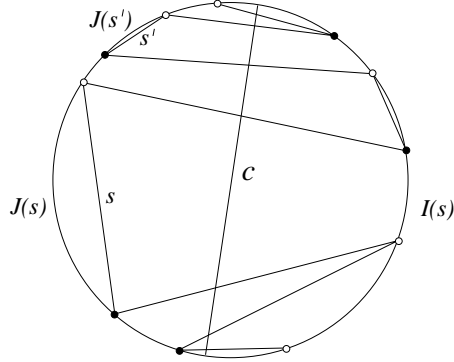
Figure 1: J(s) and J(s') are disjoint.
