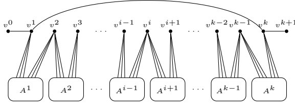
Fig. 1: Vertex gadget G_v for v \in V_i .
